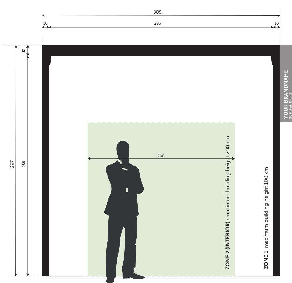
Front View
